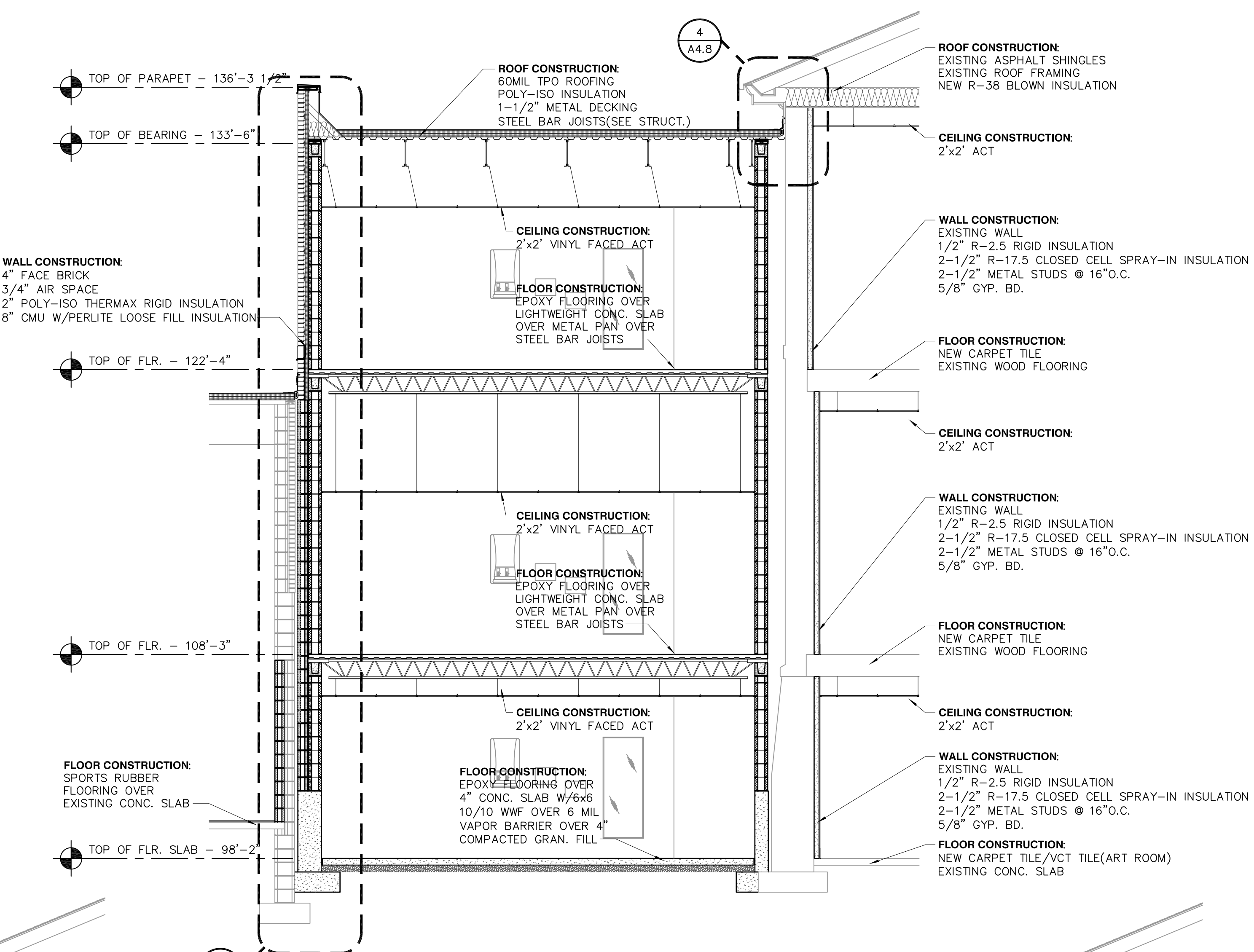
2 BUILDING SECTION 'D' SCALE: 1/4"=1'-0"
