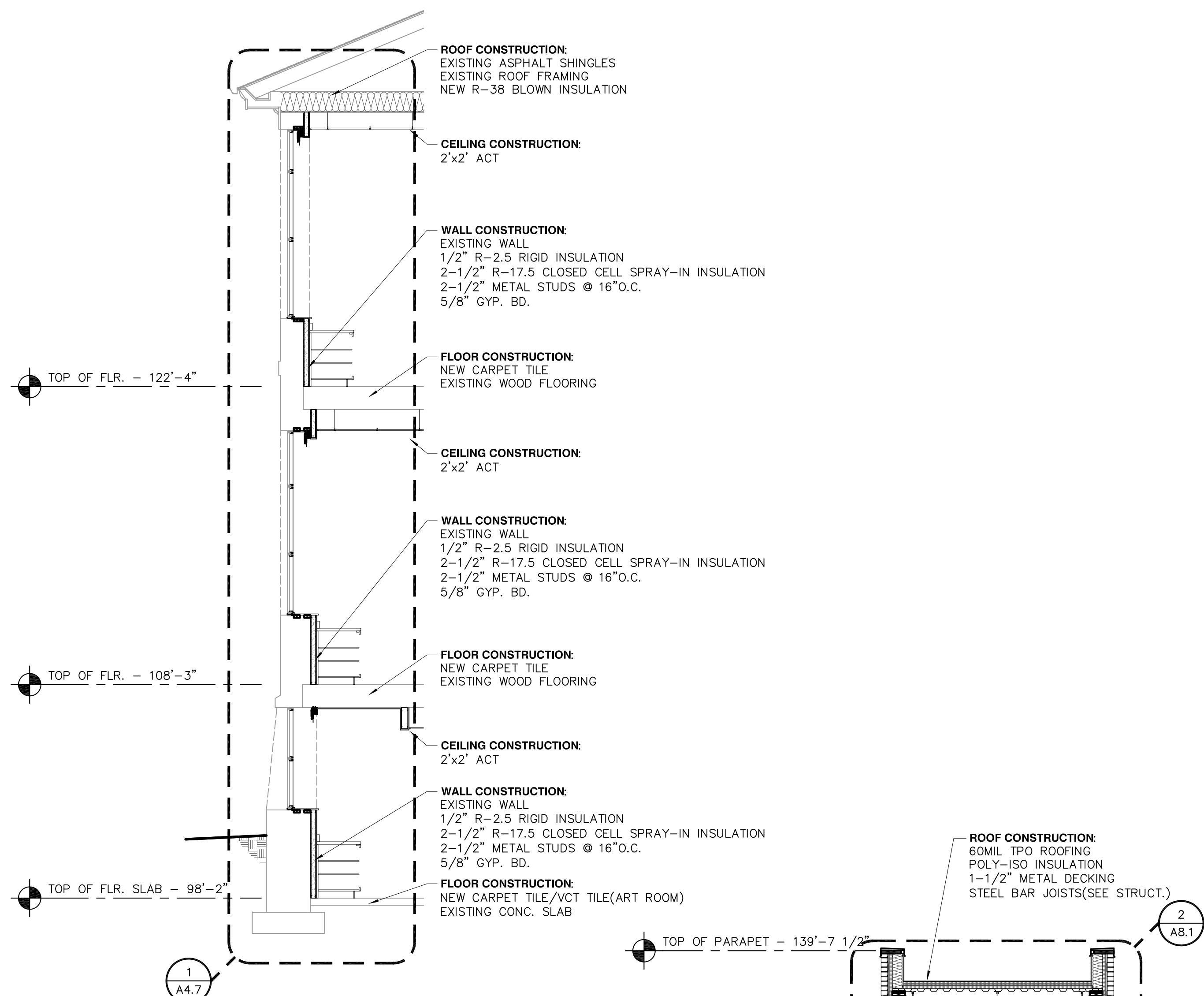
1 BUILDING SECTION 'C' SCALE: 1/4"=1'-0"
